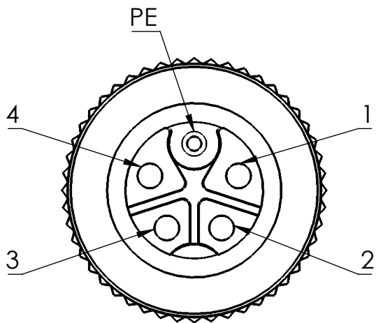
P1 M12 K-coded (Female) Front View Scale 3:1
