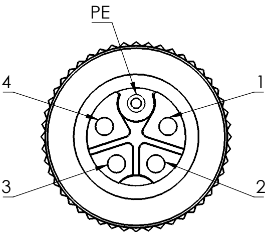
P2 M12 K-coded (Female) Front View Scale 3:1
