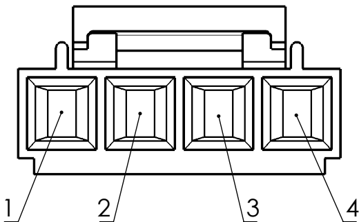
P2 Molex Sabre 4 Position (Receptacle) Wire Entry View Scale 2:1
